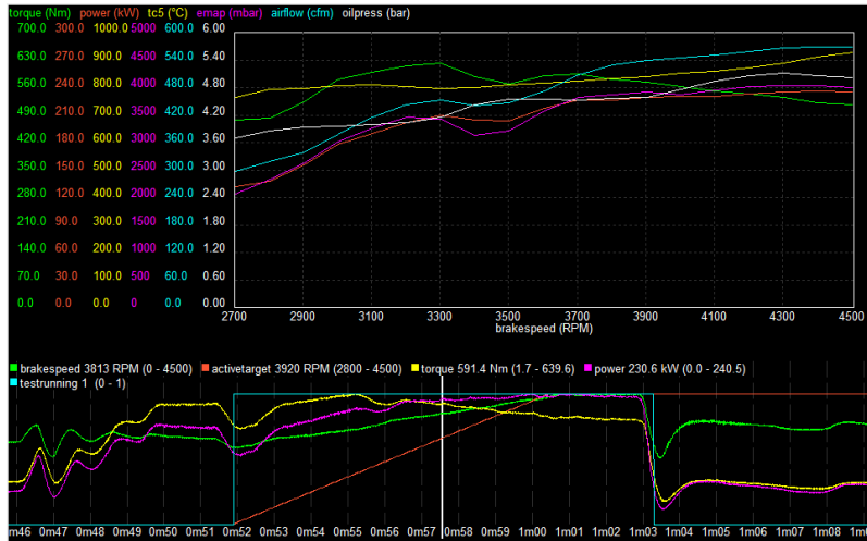
Figure 5.8: Interval report of a dyno test in graphical mode
